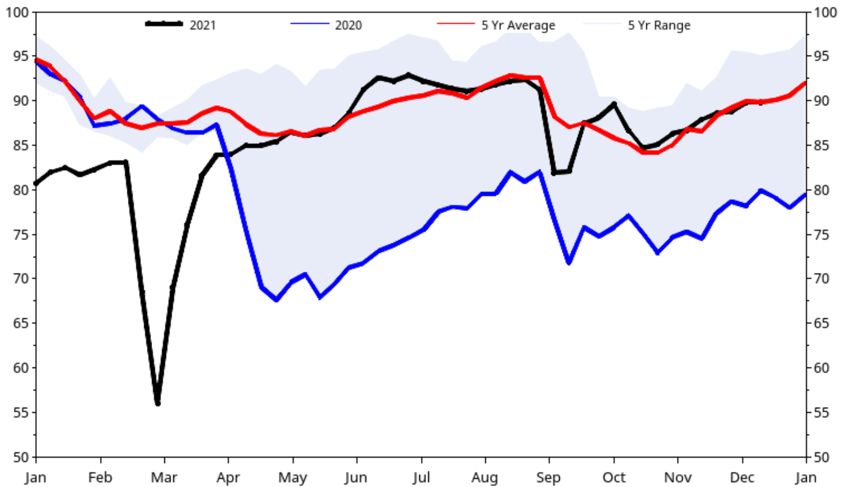
December 10, 2021 Refinery Utilization 89.80 % 0.00 Week Change
